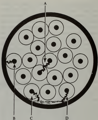
FIGURE 4-69. Cross section of an ignition harness.
